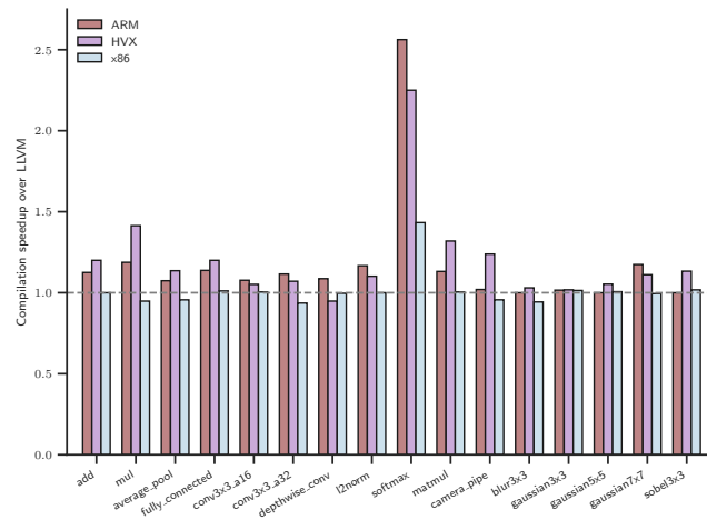
Figure 6: Compile-time speed-up over LLVM alone for the three backends. PITCHFORK improved runtime performance without compile-time cost – compile times are in fact slightly improved in most cases by passing less code to the downstream LLVM compiler.
